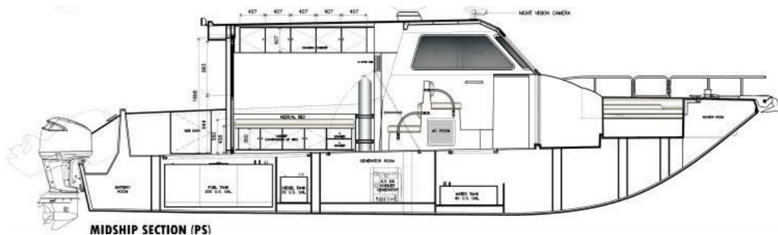
MIDSHIP SECTION (PS)
