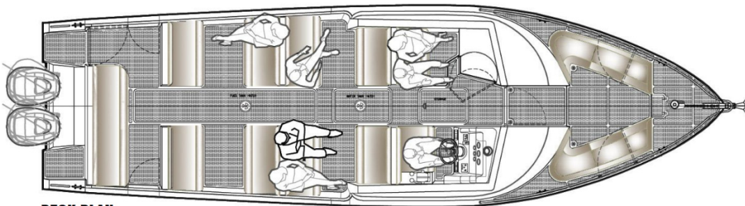
DECK PLAN
