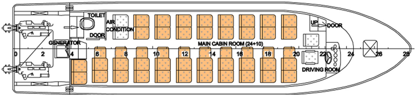
MAIN DECK AND CABIN
