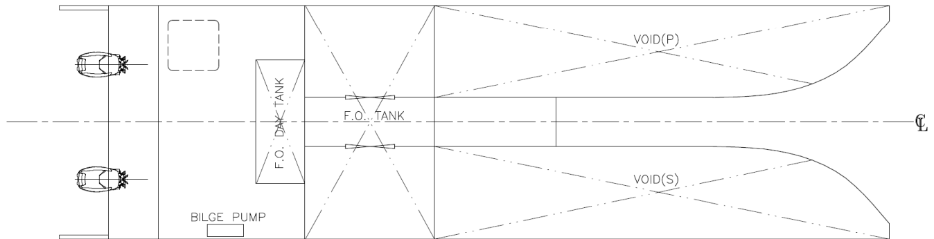
BELOW DECK PLAN
