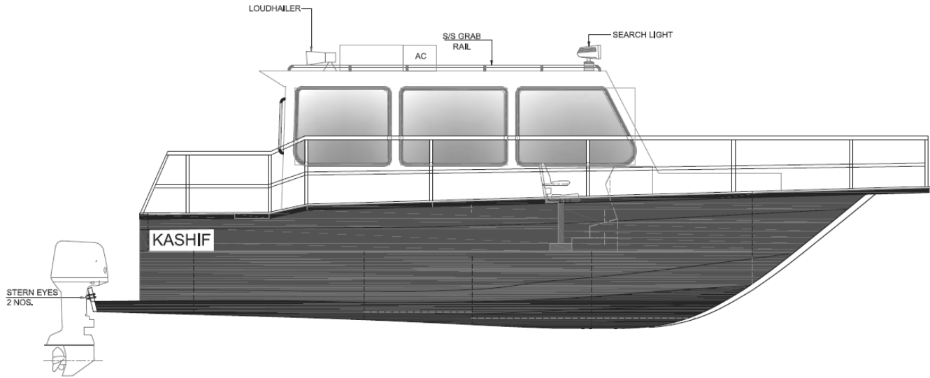
SIDE VIEW
